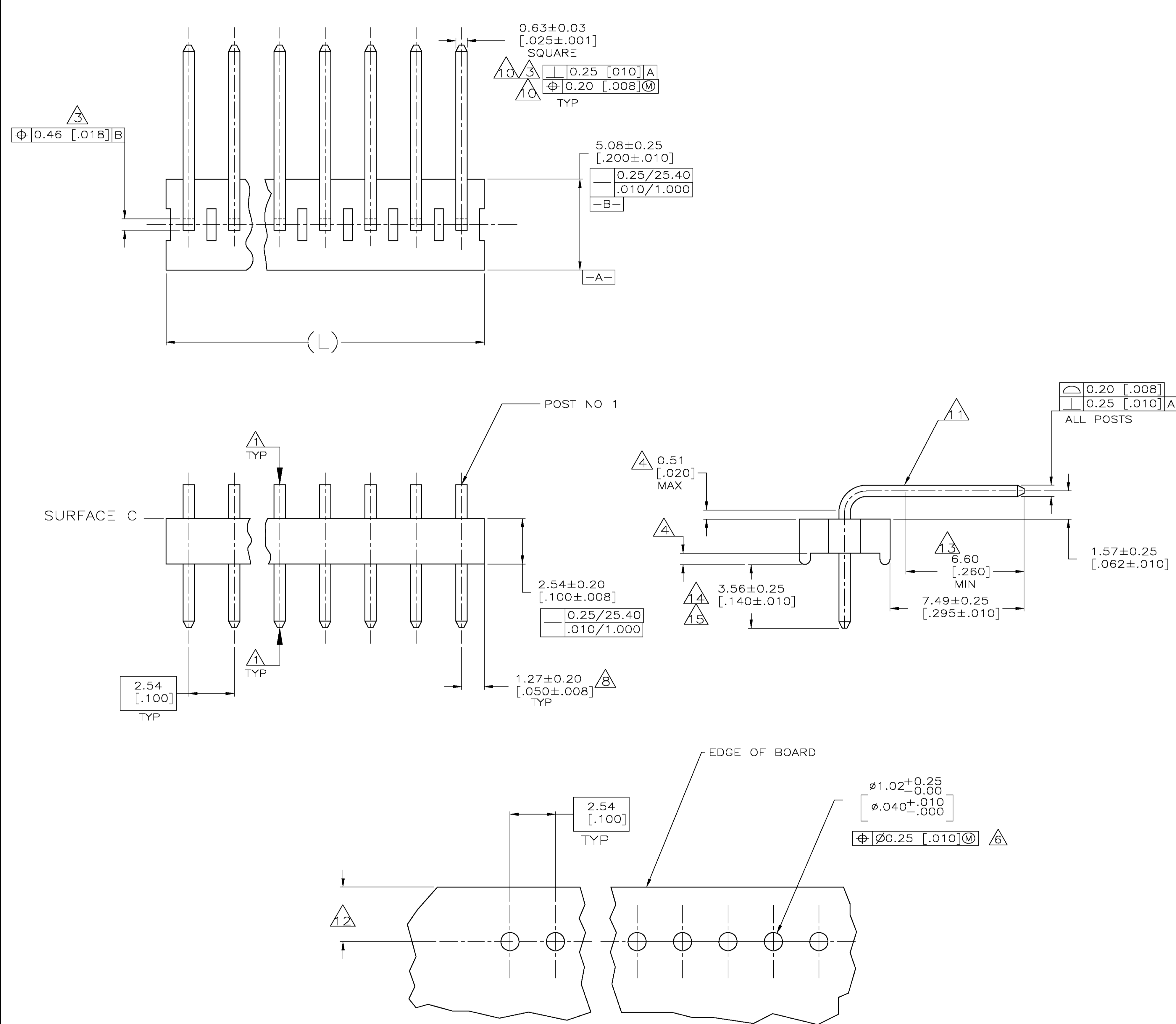
RECOMMENDED MOUNTING HOLE PATTERN FOR 1.60 [.063] THICK P.C. BOARD
